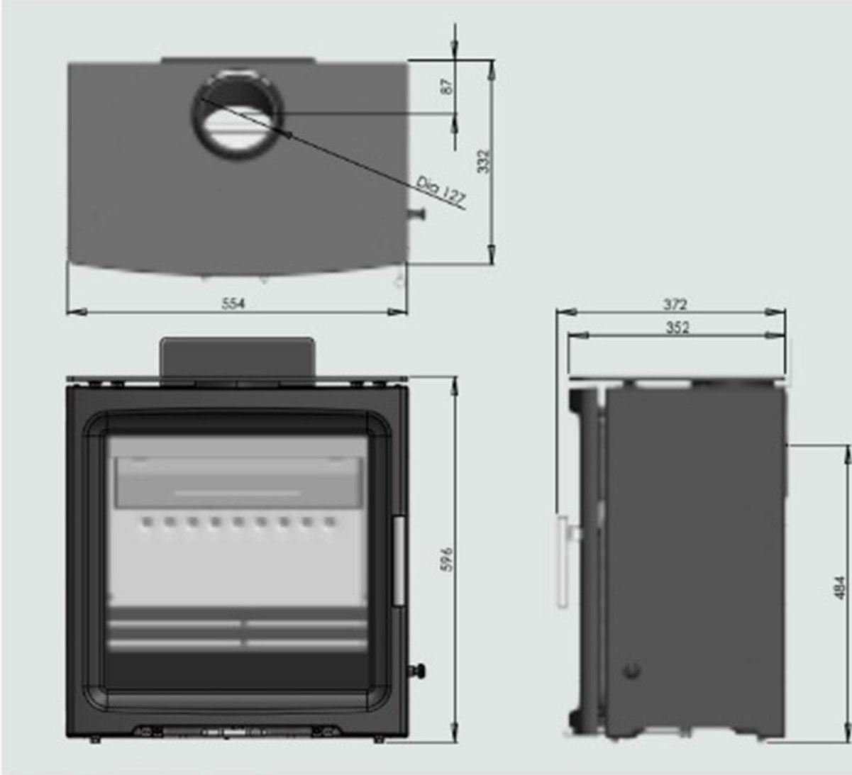
PV5W/BPV5W Slimline
